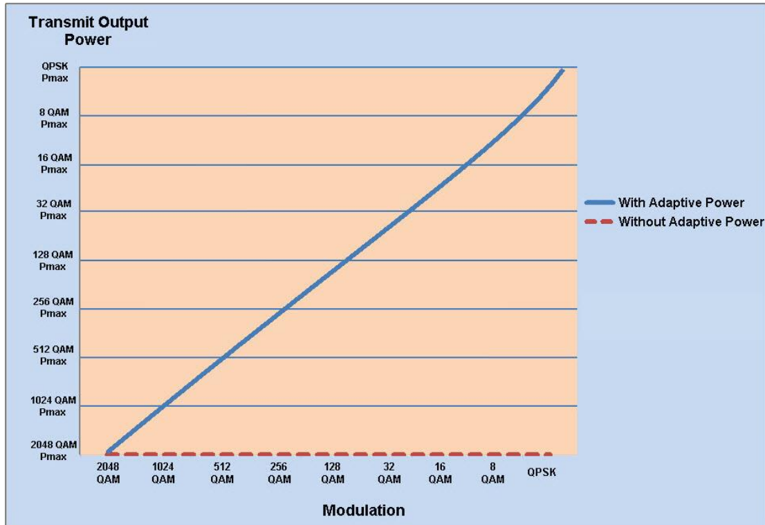
Figure 16: IP-20S ACM with Adaptive Power Contrasted to Other ACM Implementations
