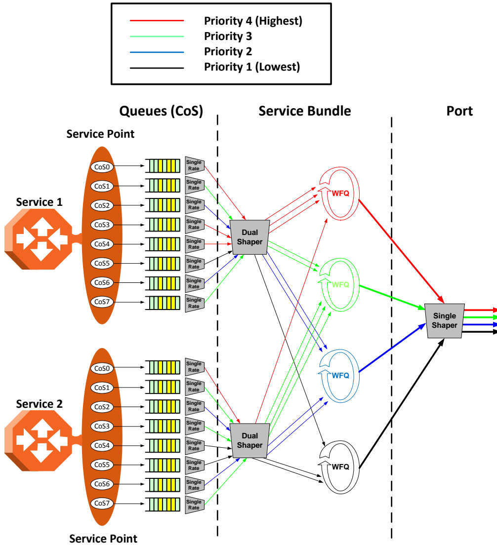
Figure 66: Detailed H-QoS Diagram
