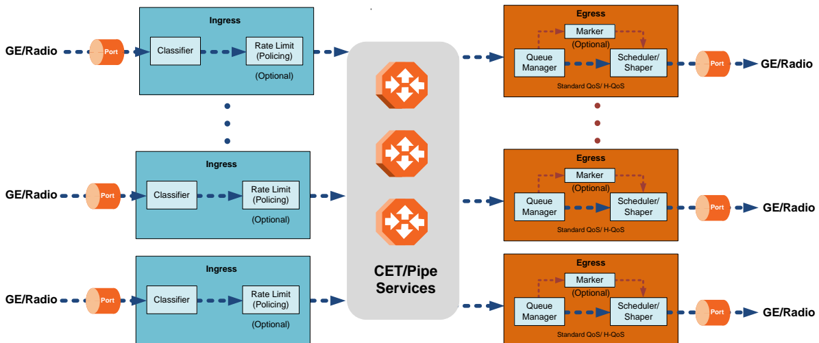
Figure 57: QoS Block Diagram
