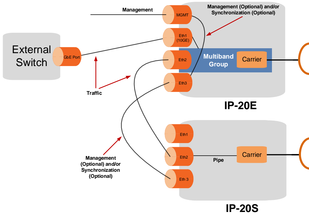
Figure 20: Multiband Operation
