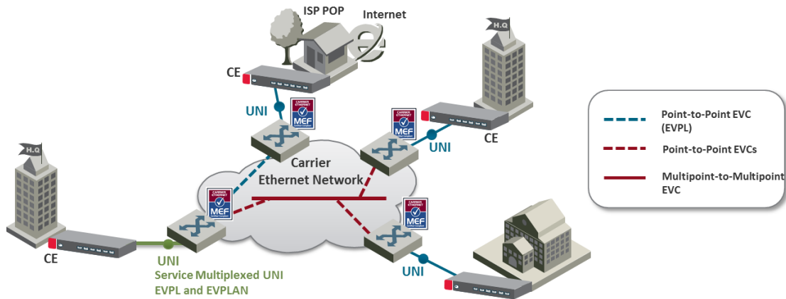
Figure 35: MEF Ethernet Virtual Private LAN Example
