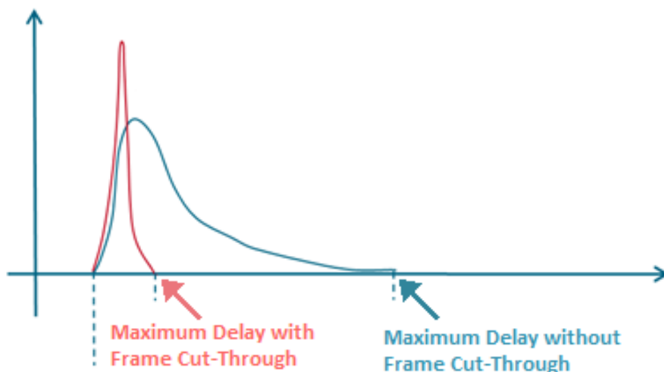
Figure 12: Propagation Delay with and without Frame Cut-Through
