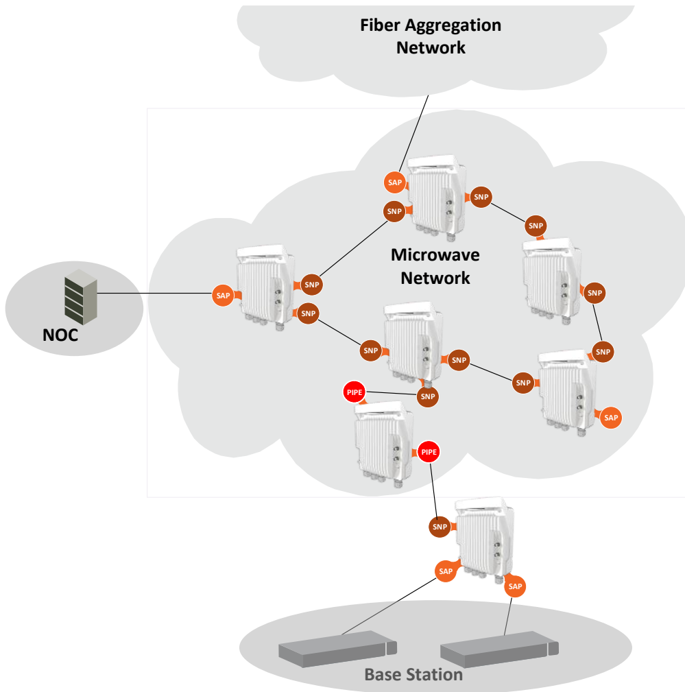
Figure 51: SAP, SNP and Pipe Service Points in a Microwave Network
