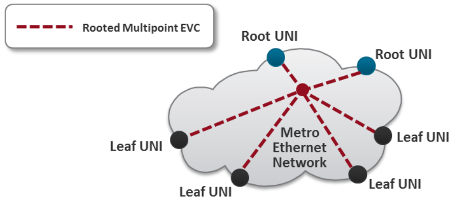
Figure 36: E-Tree Service Type Using Rooted-Multipoint EVC
