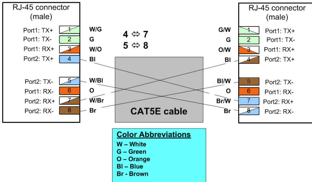
Figure 7: Protection Signaling Cable Pinouts
