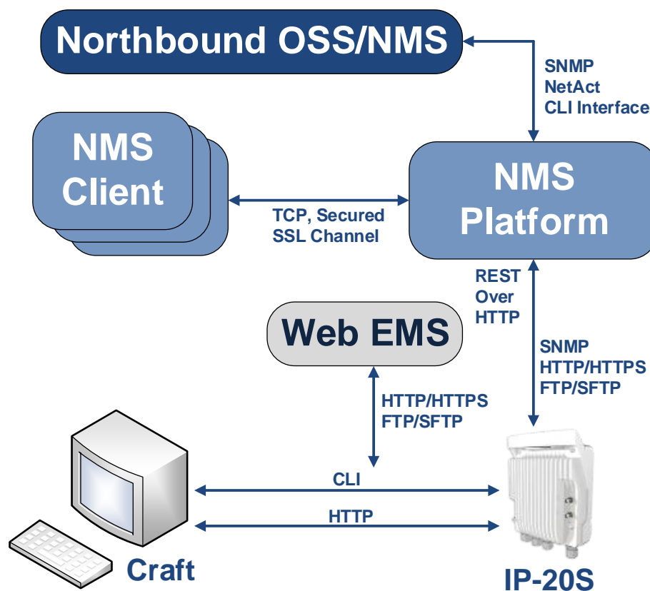
Figure 82: Integrated IP-20S Management Tools
