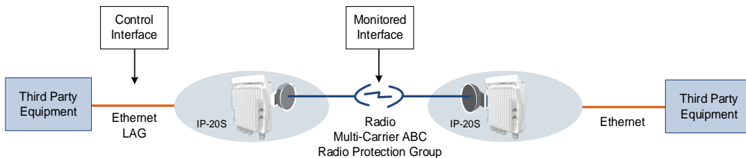
Figure 69: ABN Entity
