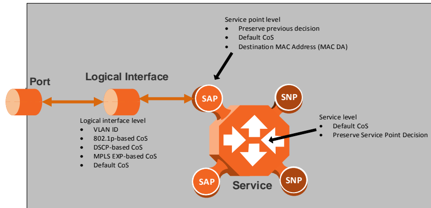
Figure 59: Hierarchical Classification
