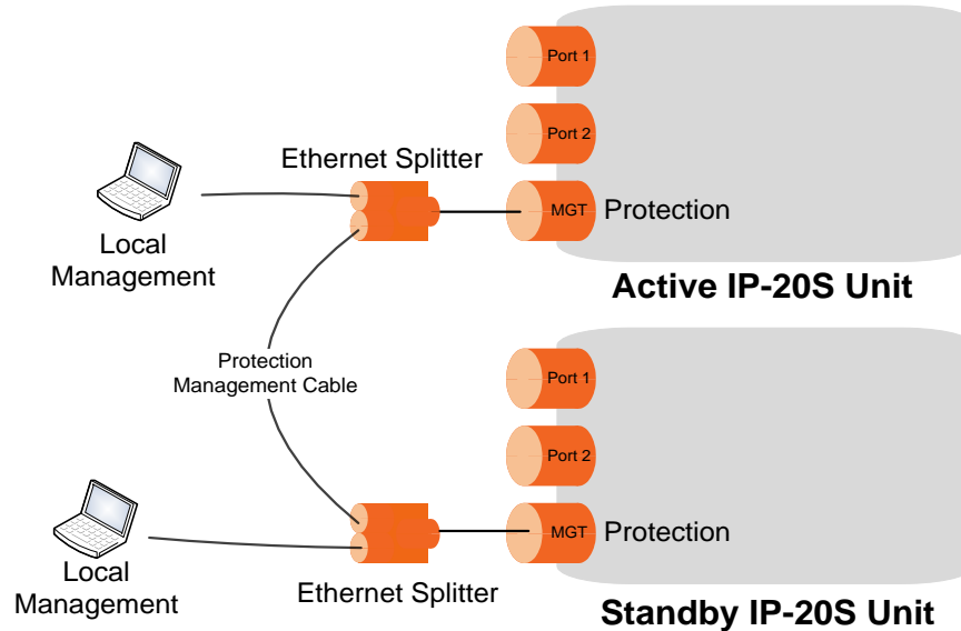
Figure 19: Internal and Local Management
