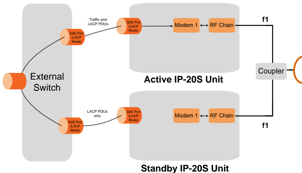
Figure 18: 1+1 HSB Protection – Line Protection Mode
