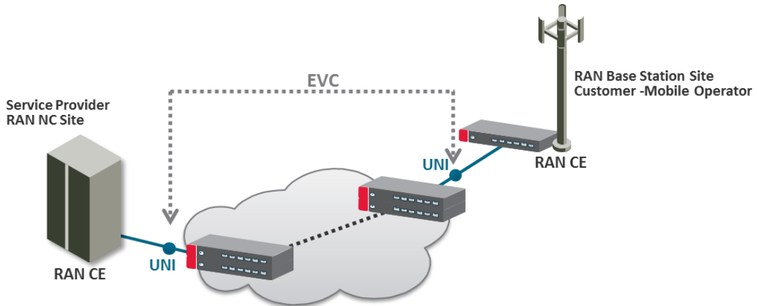
Figure 40: Mobile Backhaul Reference Model
