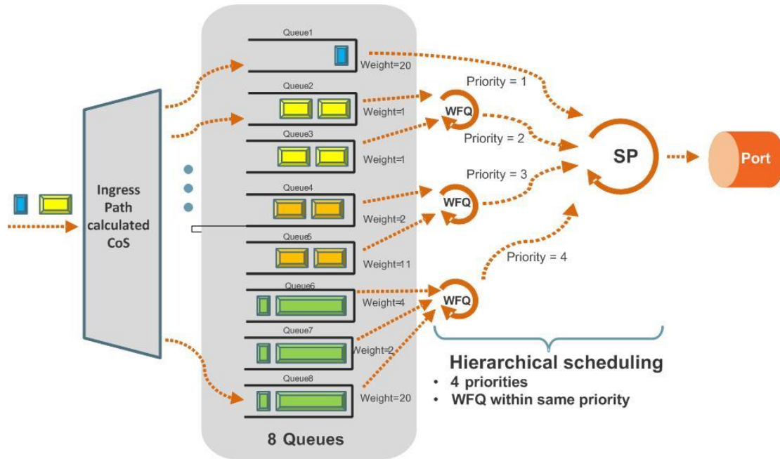
Figure 67: Scheduling Mechanism for a Single Service Bundle
