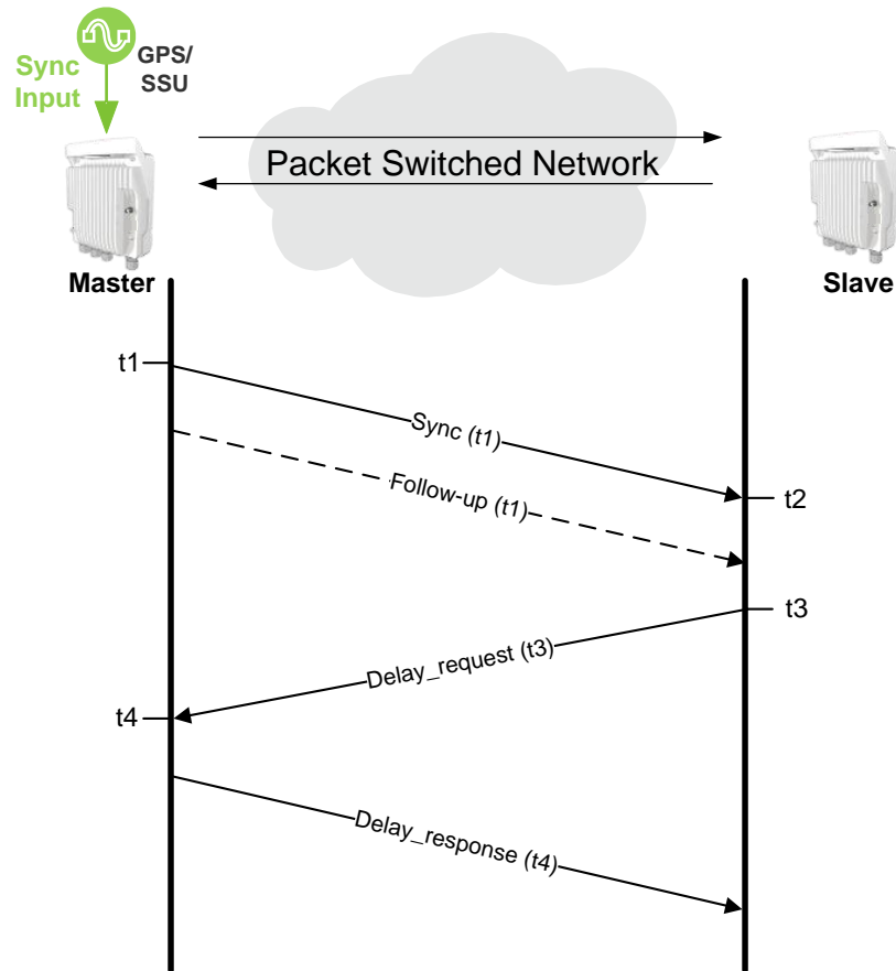
Figure 77: Calculating the Propagation Delay for PTP Packets
