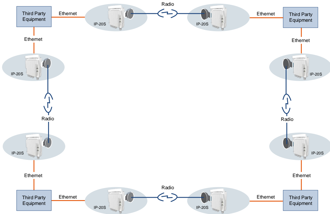
Figure 68: Network Topology with IP-20S Units and Third-Party Equipment
