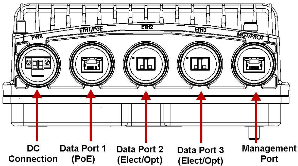
Figure 4: IP-20S Interfaces – Descriptive Labels
