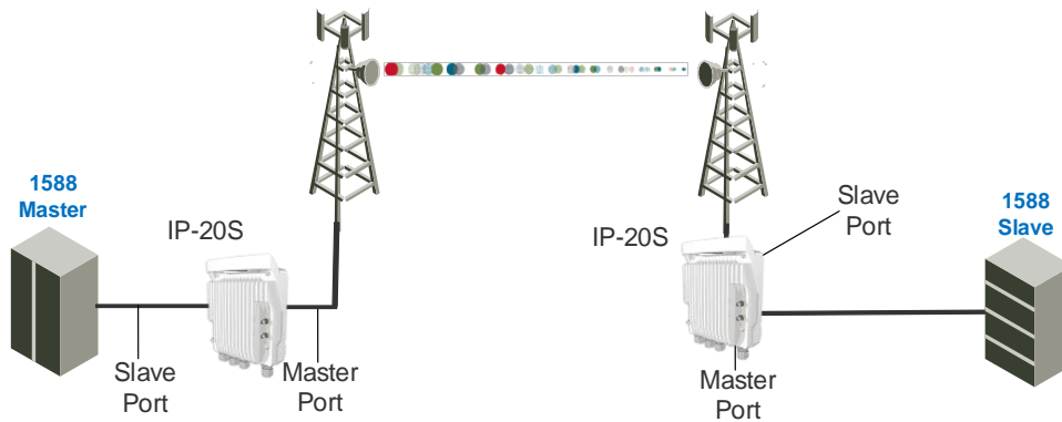
Figure 80: Boundary Clock – General Architecture
