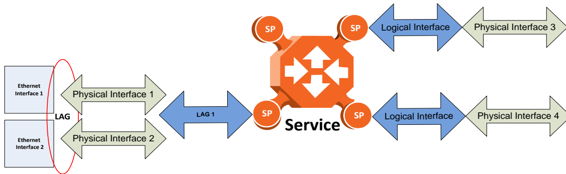
Figure 56: Relationship of Logical Interfaces to the Switching Fabric
