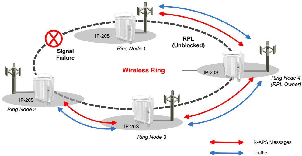
Figure 71: G.8032 Ring in Protecting State
