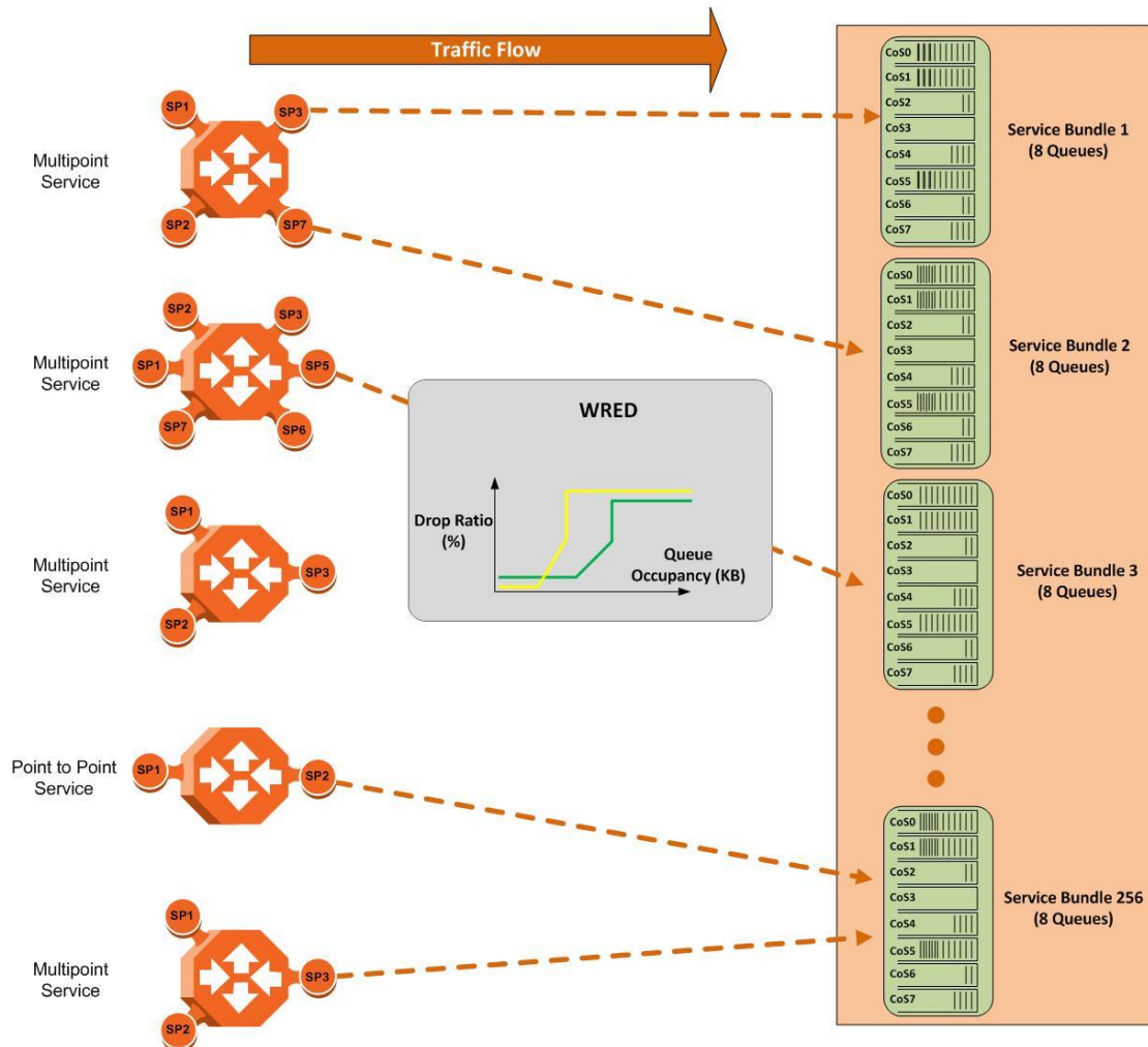
Figure 62: IP-20S Queue Manager
