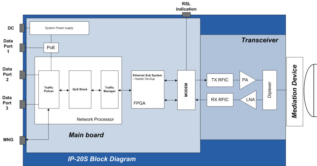
Figure 3: IP-20S Block Diagram
