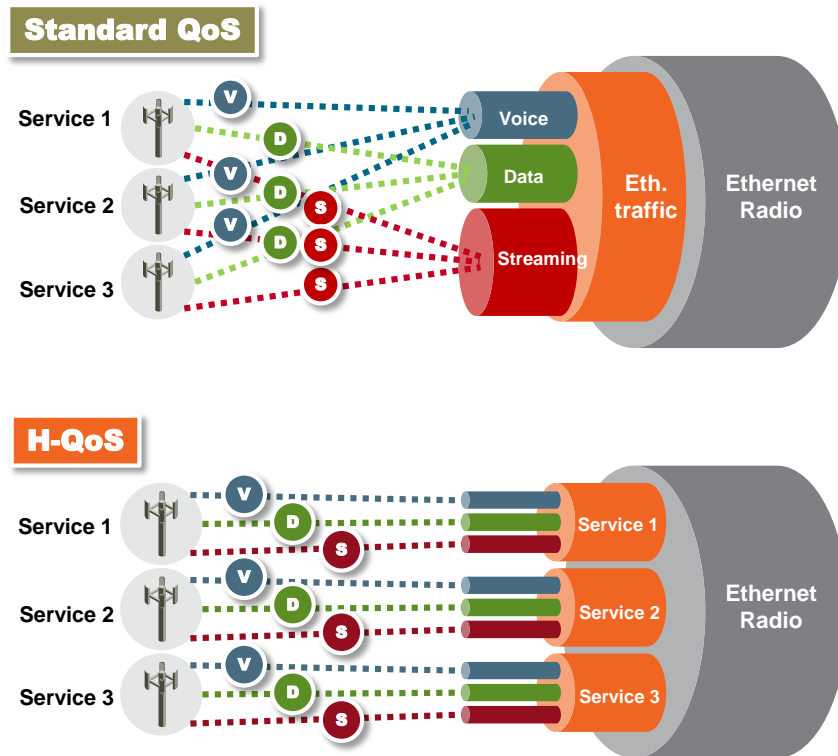
Figure 58: Standard QoS and H-QoS Comparison
