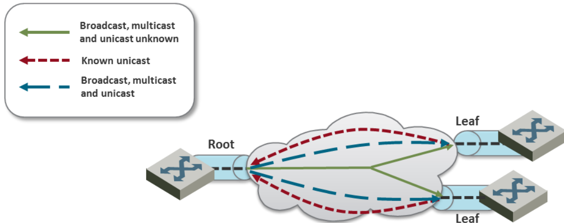
Figure 26: Rooted Multipoint EVC
