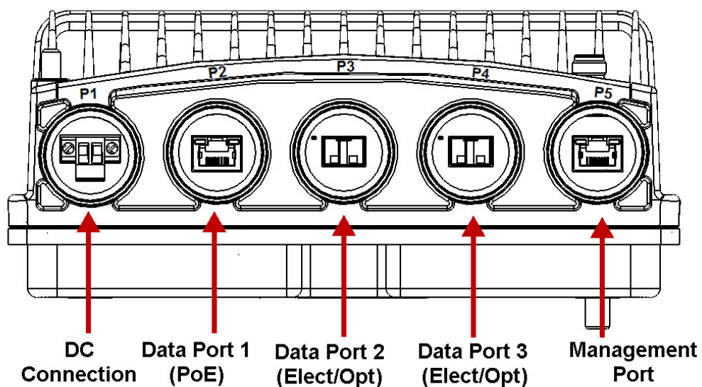
Figure 5: IP-20S Interfaces – Letter Labels
