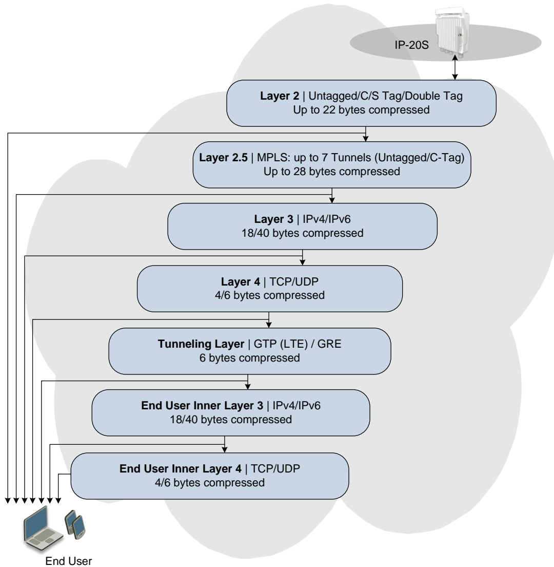
Figure 11: Header De-Duplication Potential Throughput Savings per Layer
