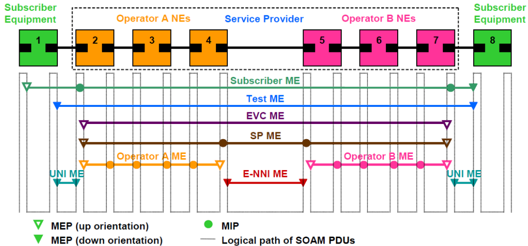
Figure 74: SOAM Maintenance Entities (Example)
