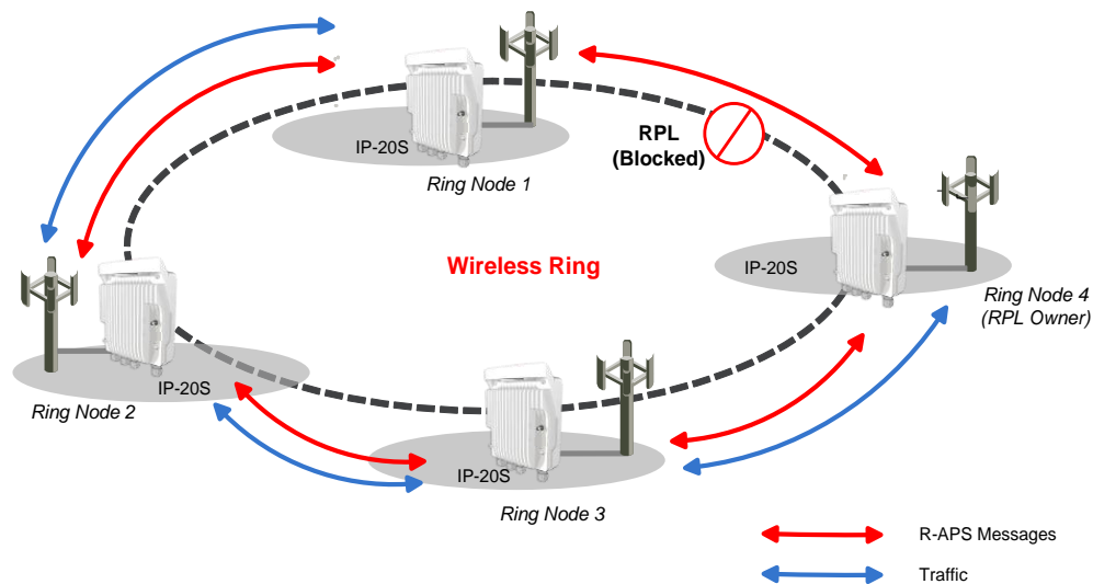
Figure 70: G.8032 Ring in Idle (Normal) State
