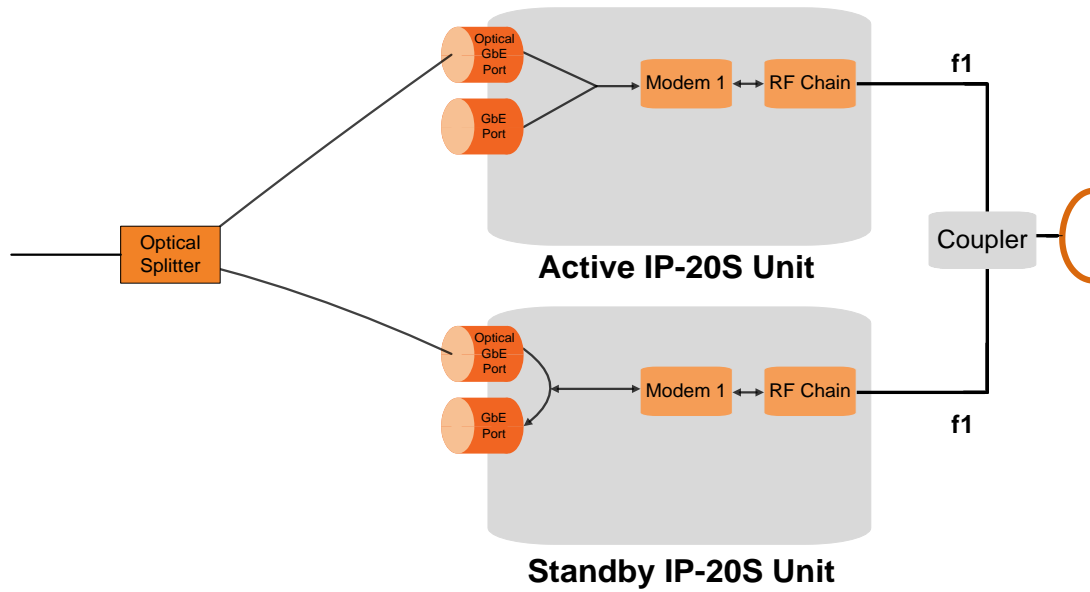
Figure 17: 1+1 HSB Protection – Split Protection Mode
