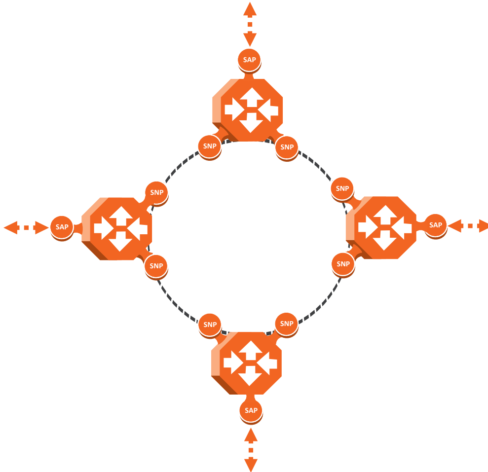
Figure 49: SAPs and SNPs
