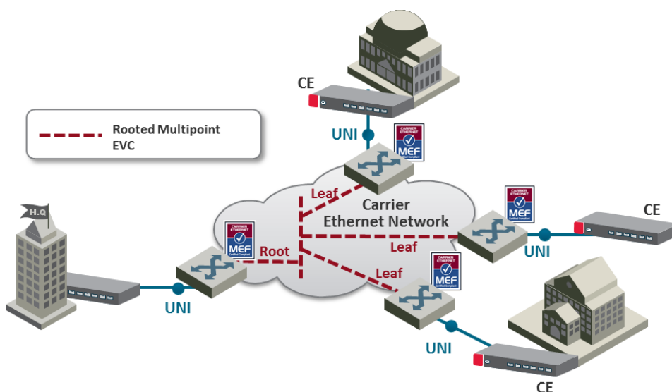
Figure 38: MEF Ethernet Private Tree Example
