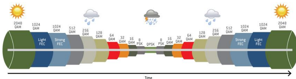
Figure 15: Adaptive Coding and Modulation with 11 Working Points
