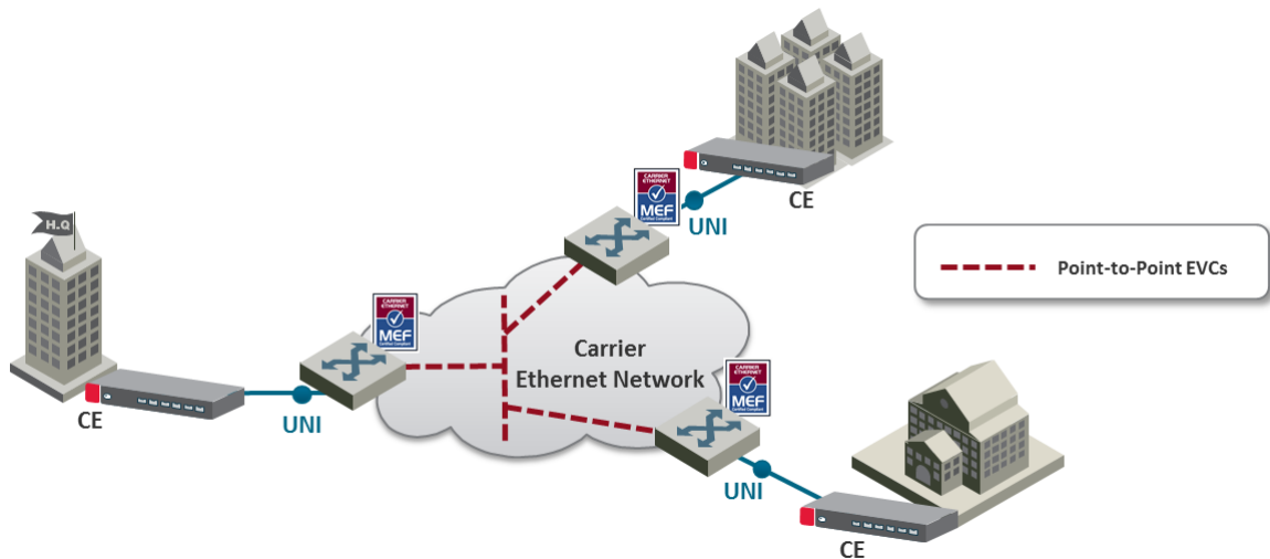
Figure 34: MEF Ethernet Private LAN Example
