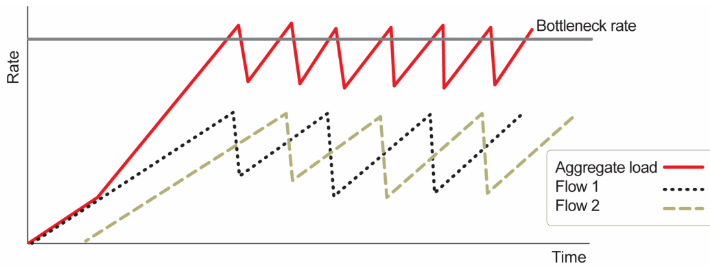
Figure 64: Random Packet Loss with Increased Capacity Utilization Using WRED
