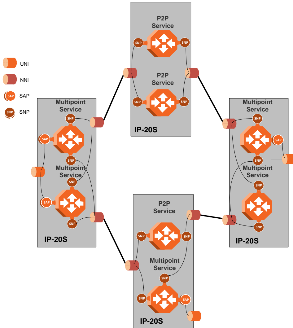
Figure 42: IP-20S Services Model
