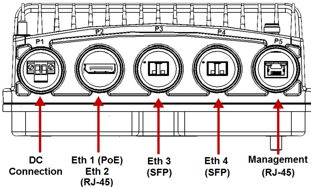
Figure 6: IP-20S Interfaces – 2E2S Model
