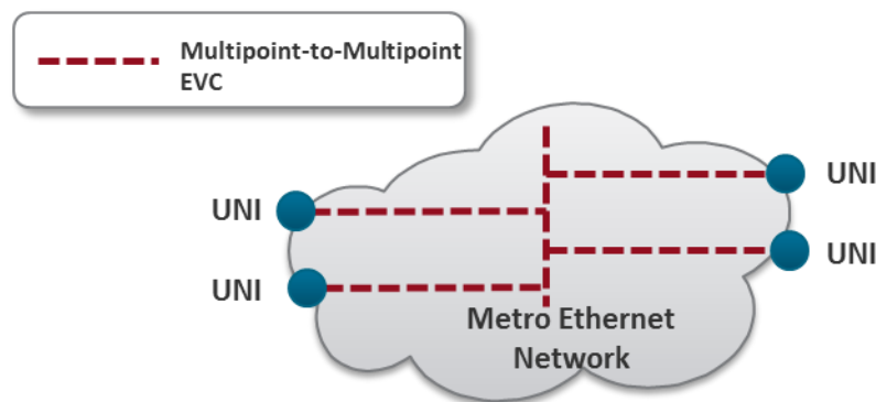
Figure 31: E-LAN Service Type Using Multipoint-to-Multipoint EVC
