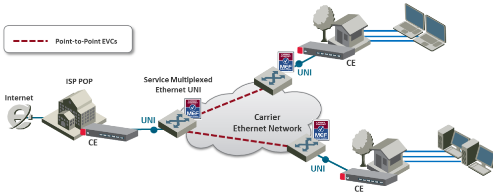
Figure 30: EVPL Application Example
