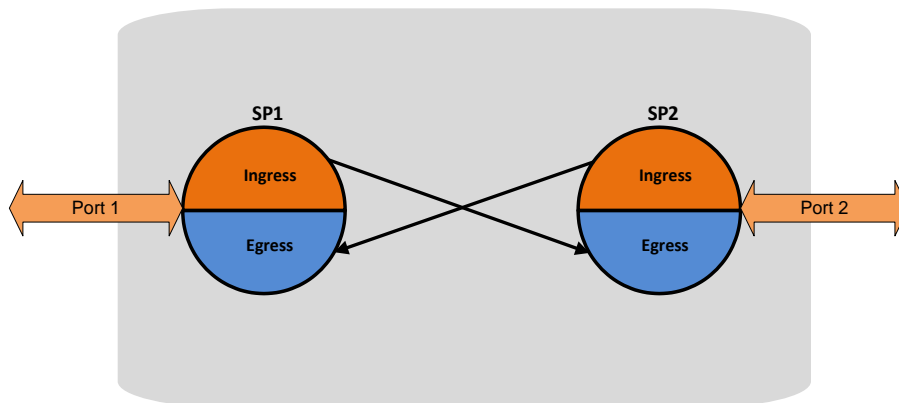
Figure 52: Service Path Relationship on Point-to-Point Service Path
