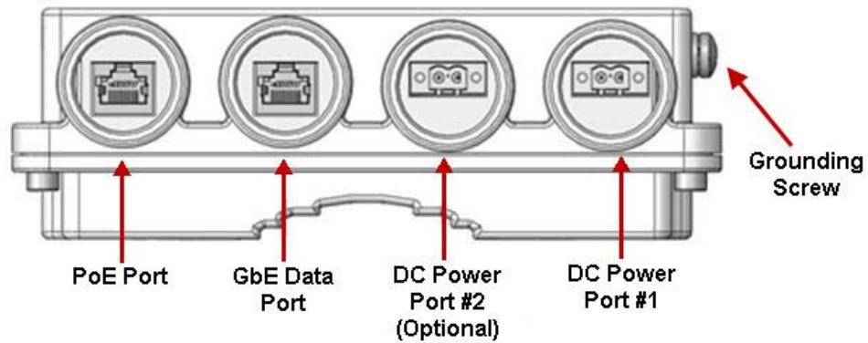
Figure 9: PoE Injector Ports
