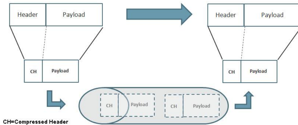
Figure 10: Header De-Duplication
