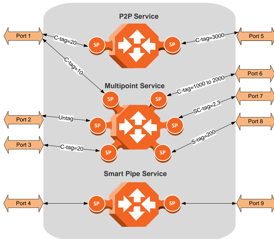
Figure 43: IP-20S Services Core
