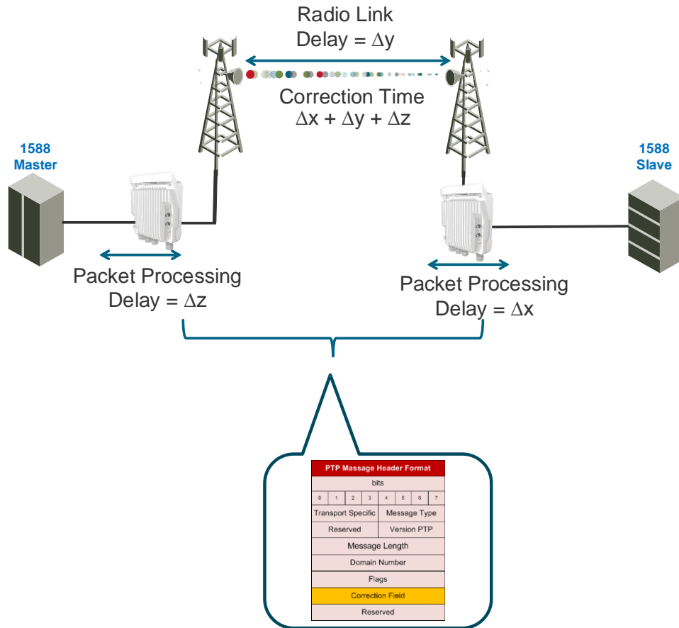
Figure 79: Transparent Clock Delay Compensation
