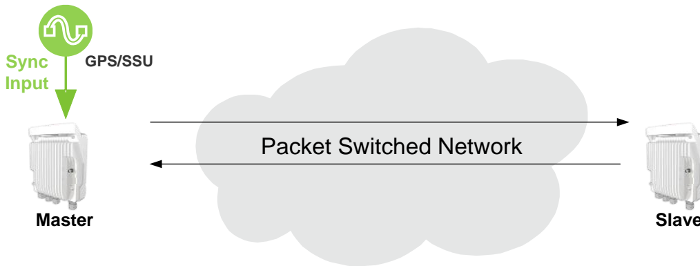
Figure 76: IEEE-1588v2 PTP Optimized Transport – General Architecture
