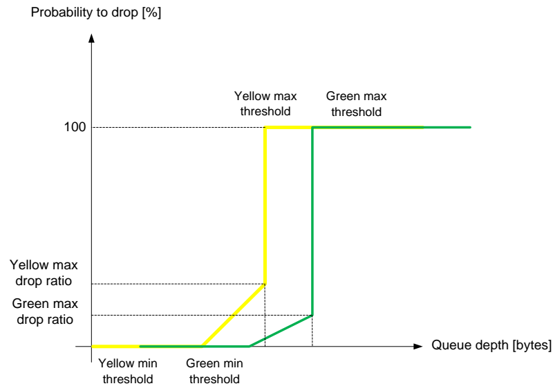
Figure 65: WRED Profile Curve
