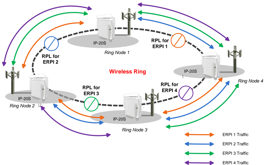
Figure 72: Load Balancing Example in G.8032 Ring
