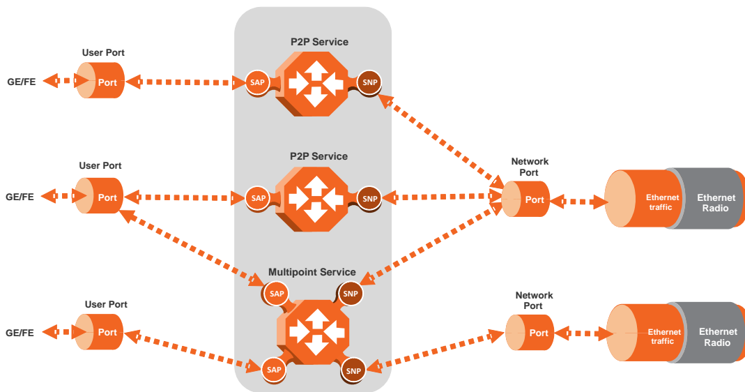
Figure 44: IP-20S Services Flow
