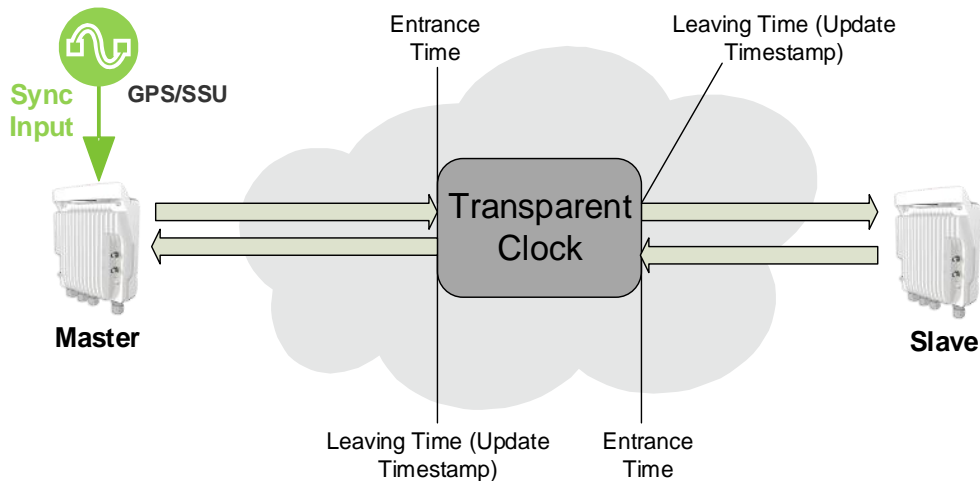
Figure 78: Transparent Clock – General Architecture
