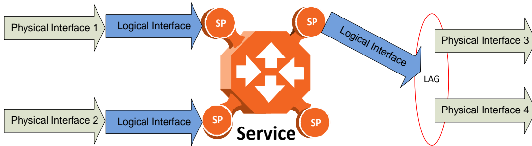
Figure 55: Grouped Interfaces as a Single Logical Interface on Egress Side
