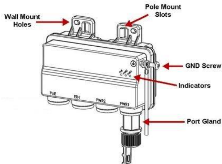
Figure 8: PoE Injector
