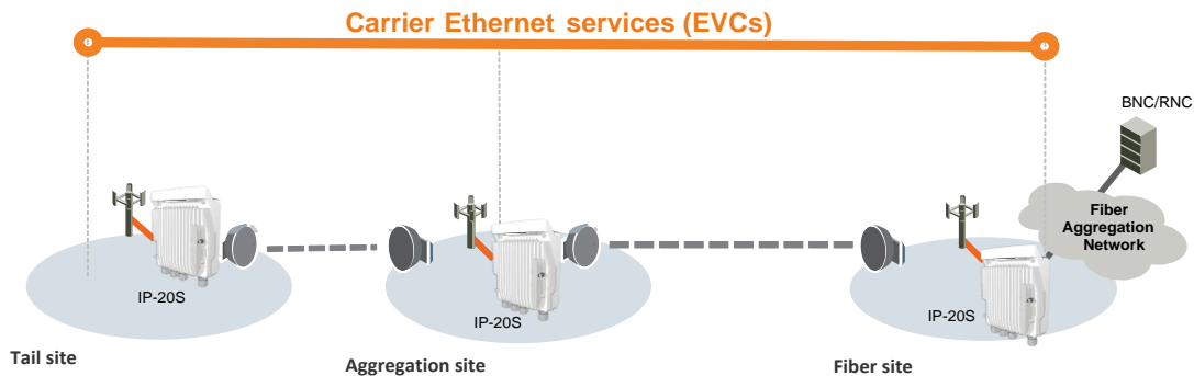
Figure 73: IP-20S End-to-End Service Management
