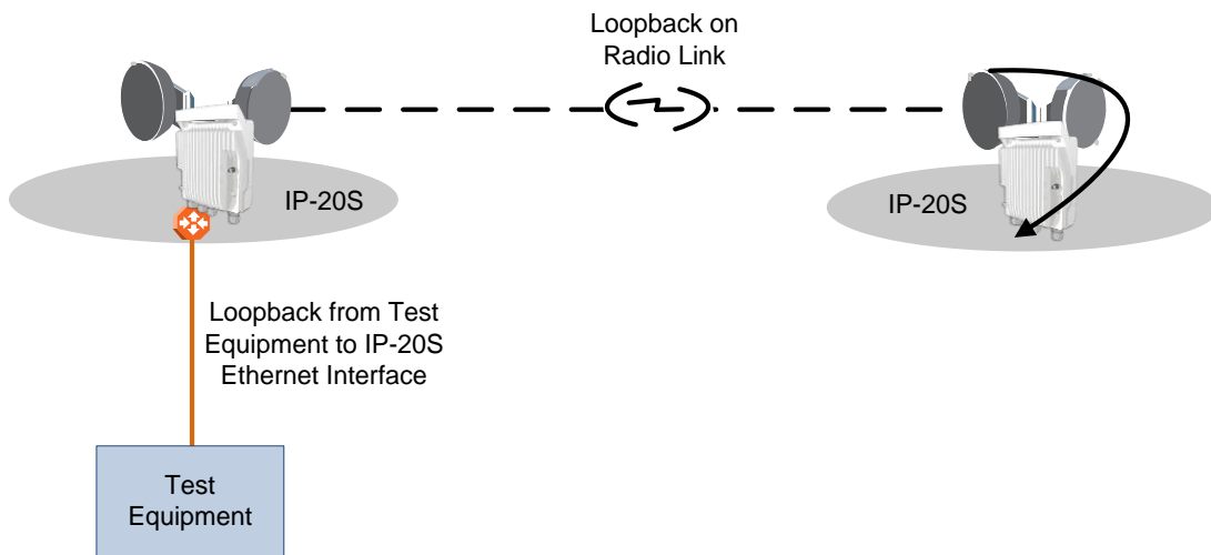
Figure 75: Ethernet Line Interface Loopback – Application Examples
