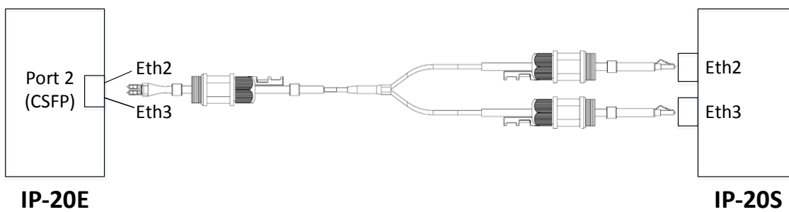
Figure 21: Multiband Cable for Use with CSFP Port
